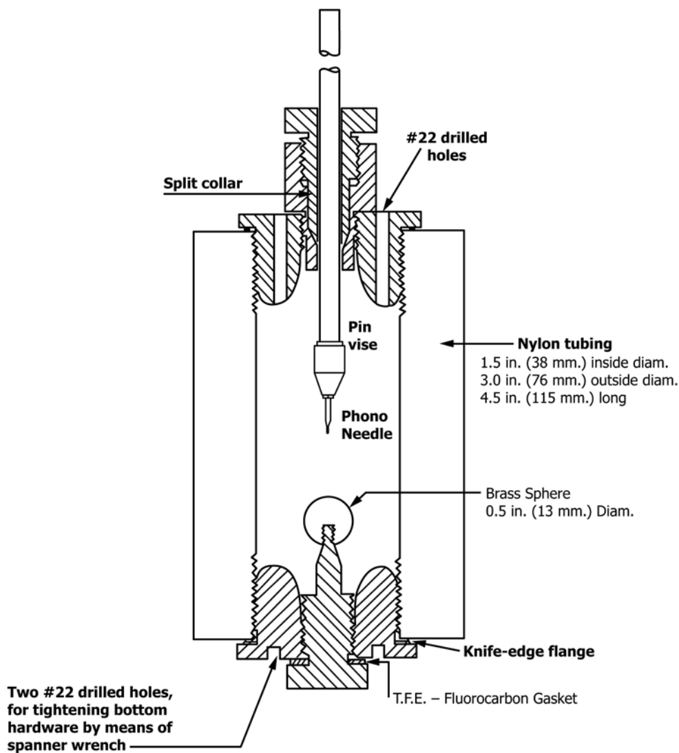
FIG. 1 Test Cell
